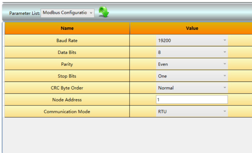
Figure 4.6 Modbus channel parameter configuration interface
