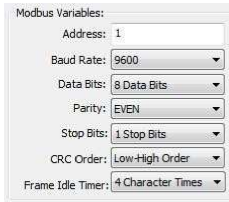
Figure 2.6 Modbus Communication Parameters
