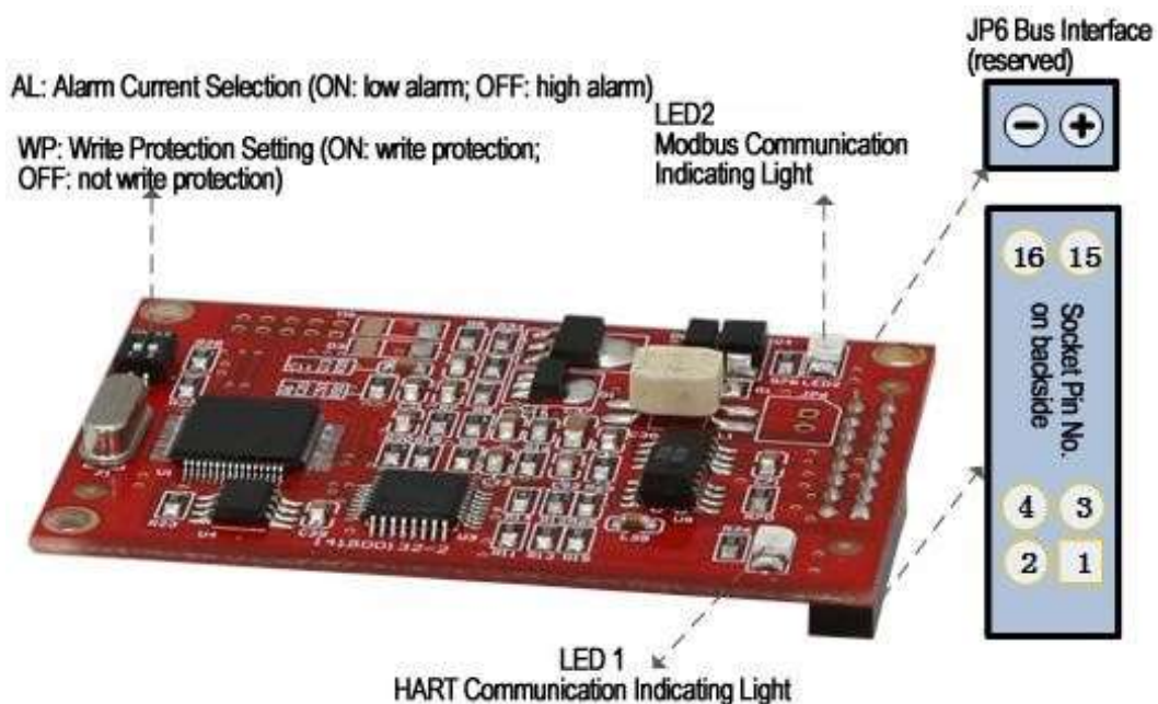
Figure 1.3 Hardware User Interface Diagram
